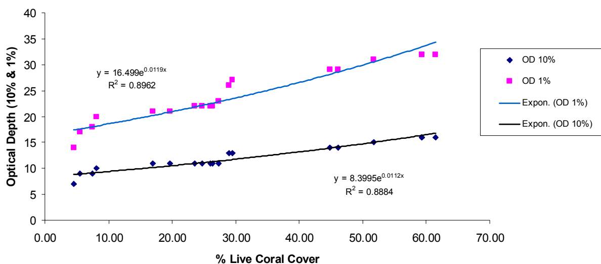
Figure 17. Relationship between the optical depth of 1% and 10% of the subsurface values, and the percent live coral cover.
